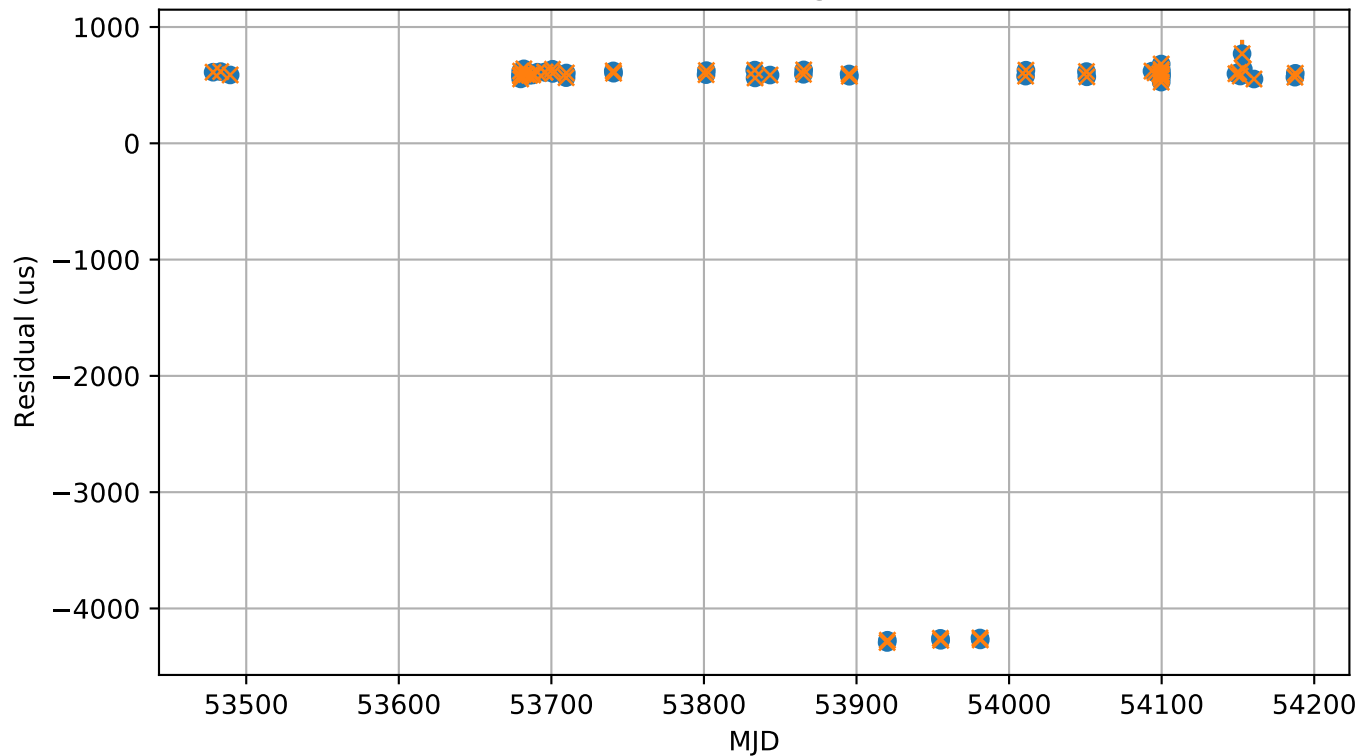
1748-2021E Timing Residuals
