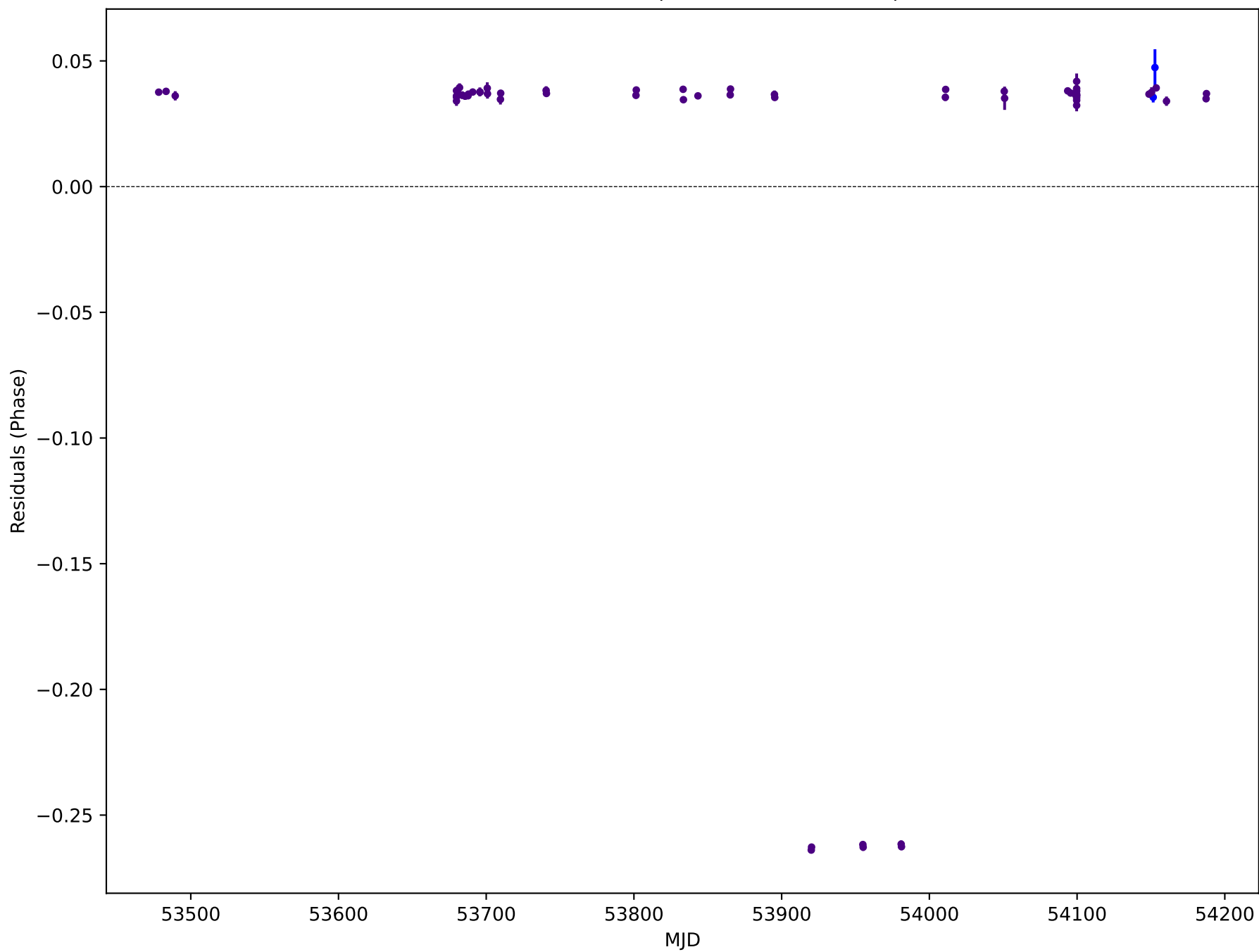
Postfit Residuals (Number of TOAs: 62)
